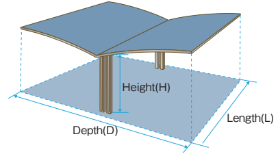
M+Y Connection
