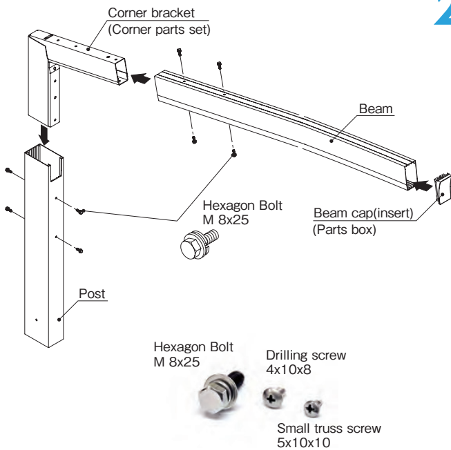
Posts - Corner Brackets - Beam connections
