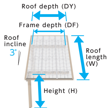
Cantilever type
